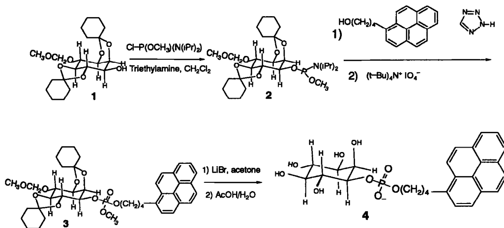
Scheme I. Synthesis of 4-(1-pyreno)butylphosphoryl- myo -inositol.
